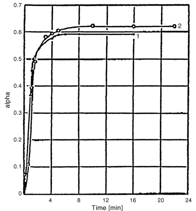
Fig. 4. Dependence of the Level of Hydrolysis of SiF 6 2- on Time. (Westendorf Figure 16). (1) 6.45 ppm of F - (5.7 × 10 -4 M of MgSiF 6 ). (2) 1.14 ppm of F - (1.01 × 10 -4 M of MgSiF 6 ). Hydrolysis is initially rapid; no more change occurred after 15 minutes.
